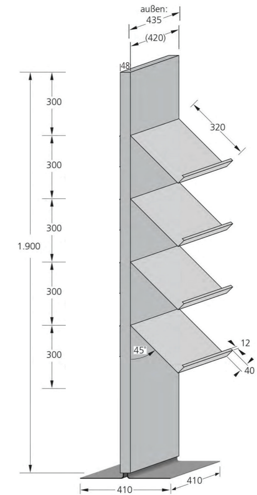
QMT 19042 with 4 shelves one-sided
