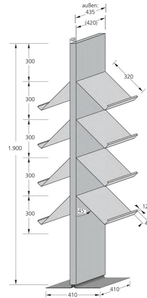
QMT 19042 with 4 shelves per side
